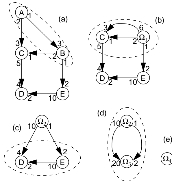
Figure 6. An illustration of APGAN.
