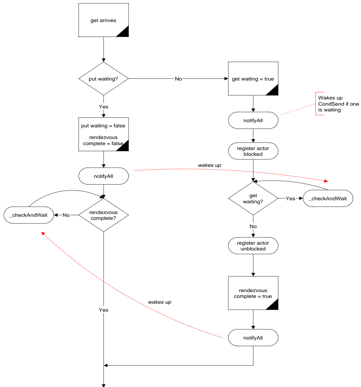
FIGURE 11. Rendezvous algorithm
