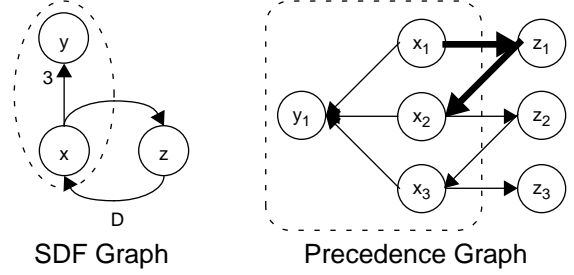
Figure 4: Example in violation of condition 3. A cycle is introduced in the precedence graph.
